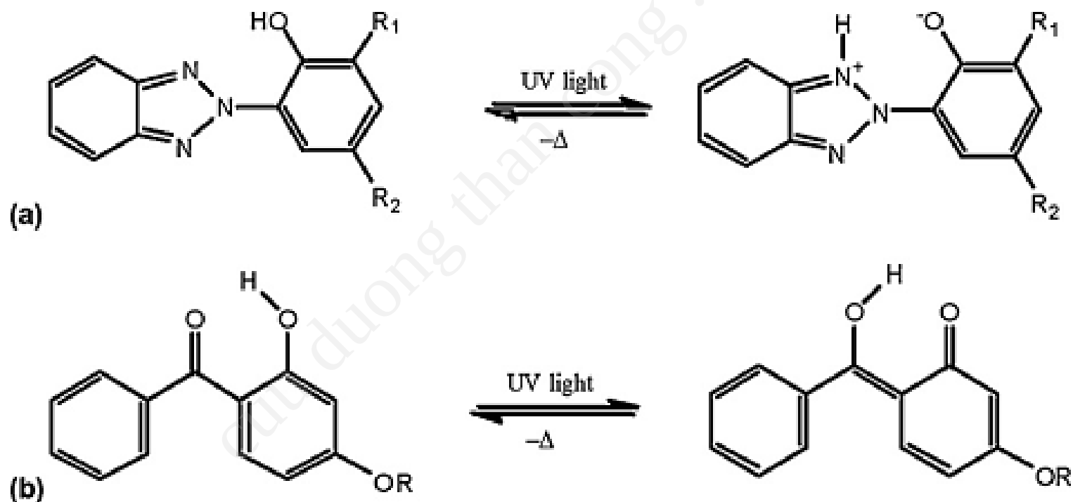
Fig. 24. Keto-enol tautomerism of benzotriazole (a) and benzophenone (b).
