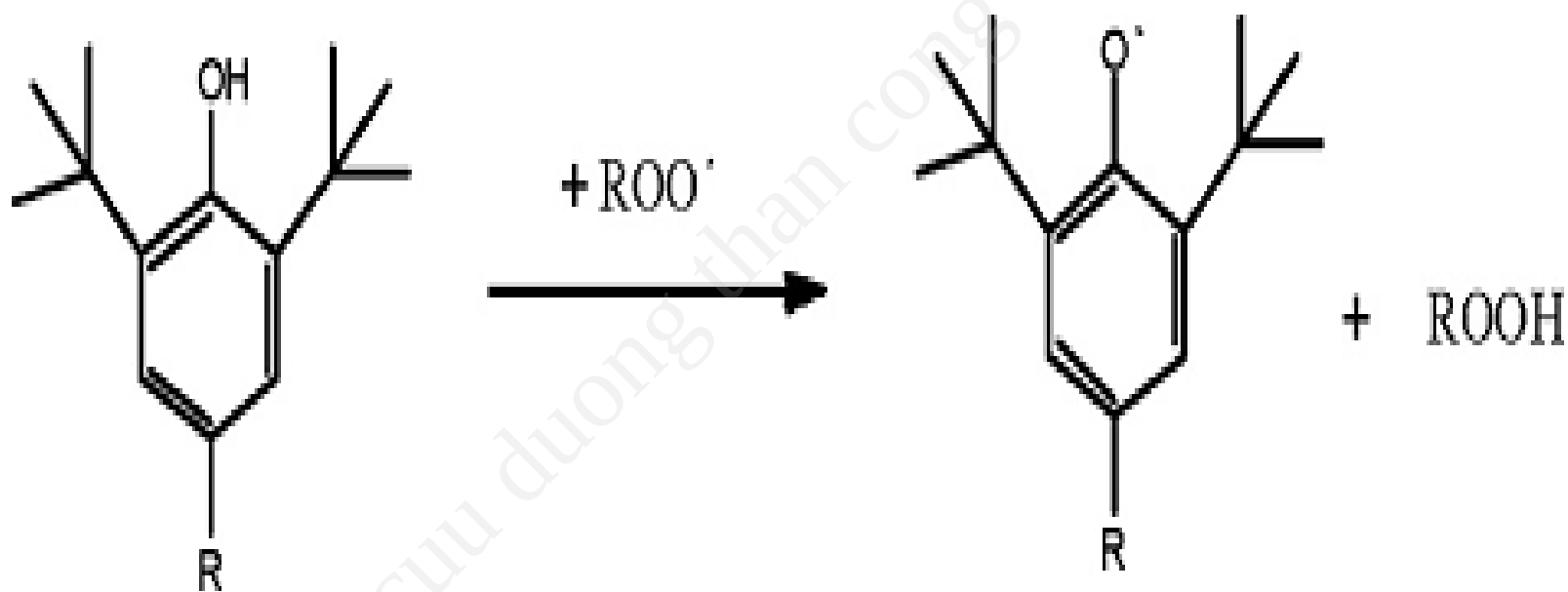
Fig. 25. Deactivation of peroxy radicals by hindered phenols.
