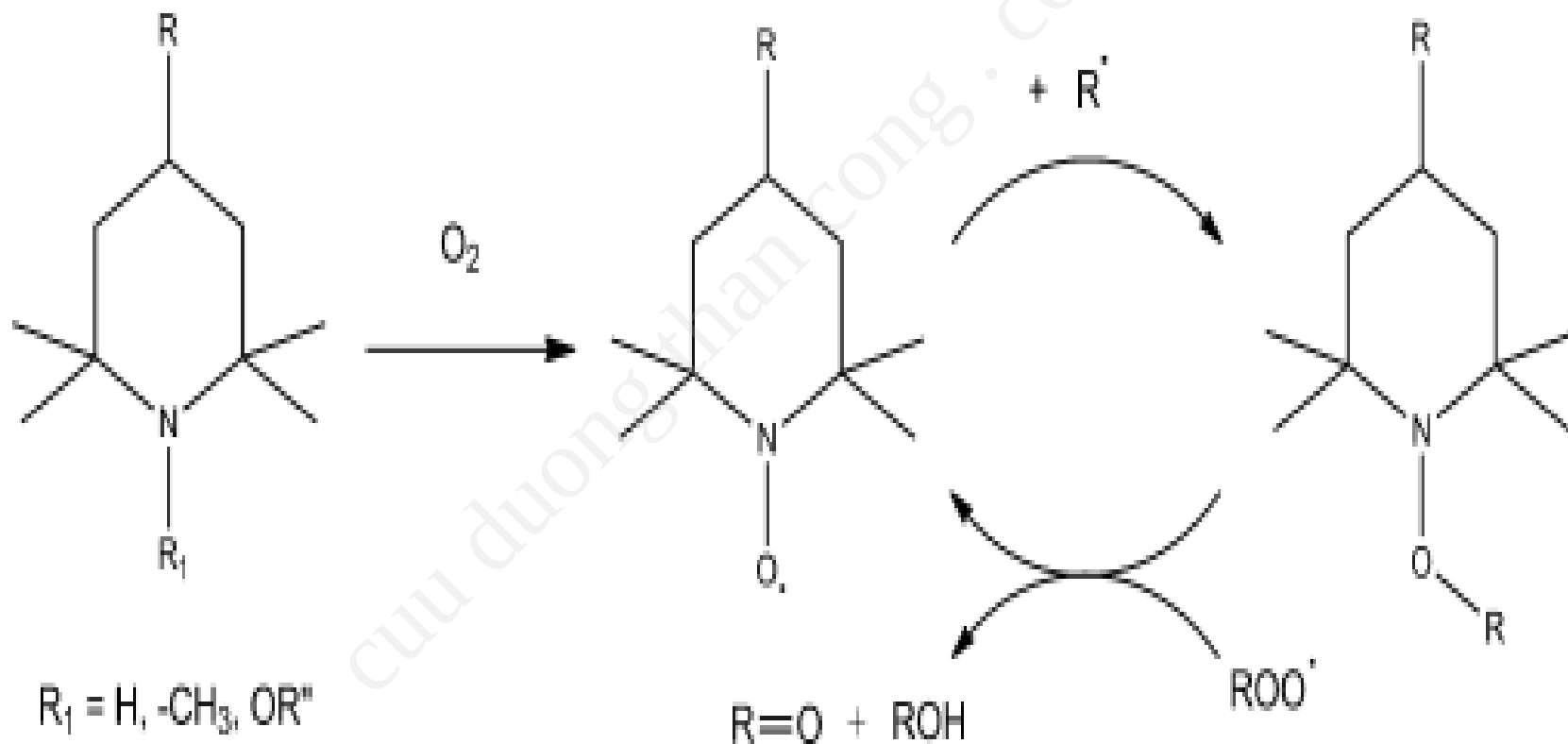
Fig. 27. Stabilisation mechanism of HALS.
