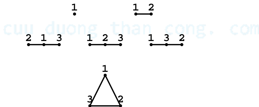
Fig. 3.1: The six labeled, connected graphs of \leq 3 vertices.
