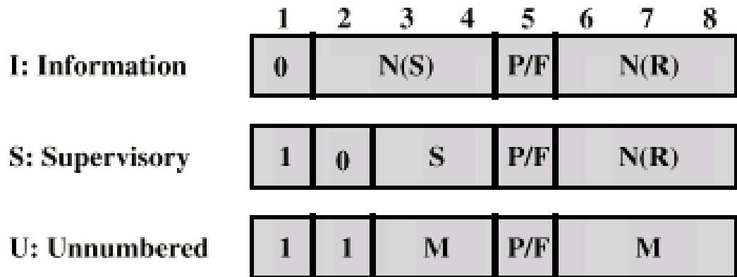
(c) 8-bit control field format cuuduongthancong.com
