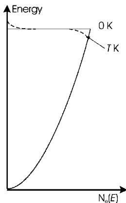
Figure 2.32 The population density, N_e(E) , for free electrons in an energy band at 0 K and a higher temperature, T K
