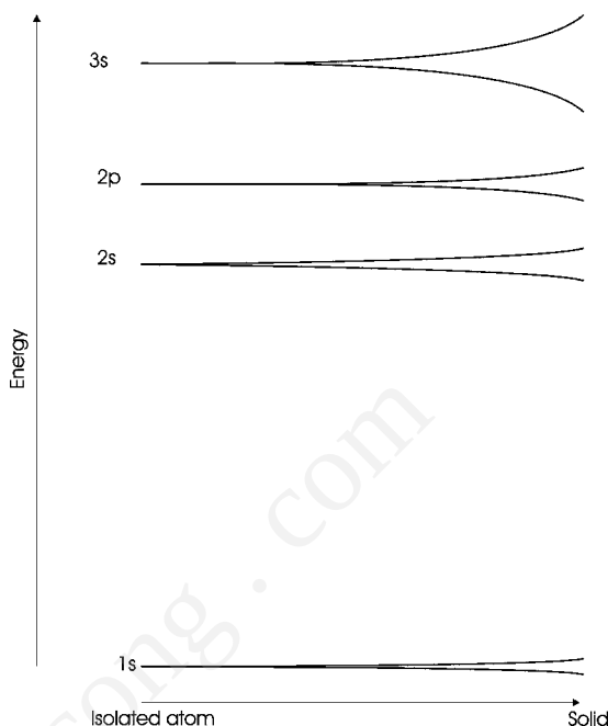
Figure 2.25 The development of energy bands from atomic orbitals for sodium metal. Isolated atoms (left-hand side) have sharp energy levels. In a solid, these are broadened into energy bands. Outermost orbitals broaden more than inner orbitals
