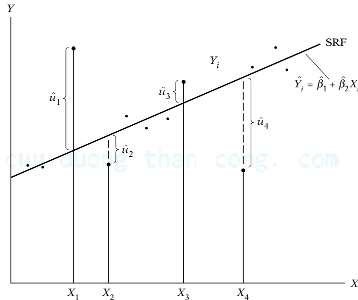
FIGURE 3.1 Least-squares criterion.
