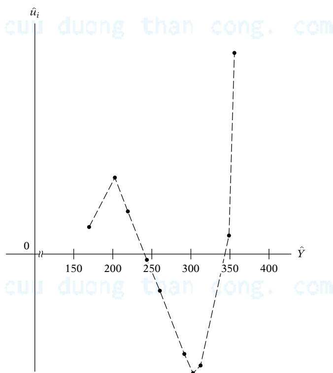
FIGURE 13.2 Residuals \hat{u}_i and estimated Y from the linear cost function: Y_i = \lambda_1 + \lambda_2 X_i + u_i .
