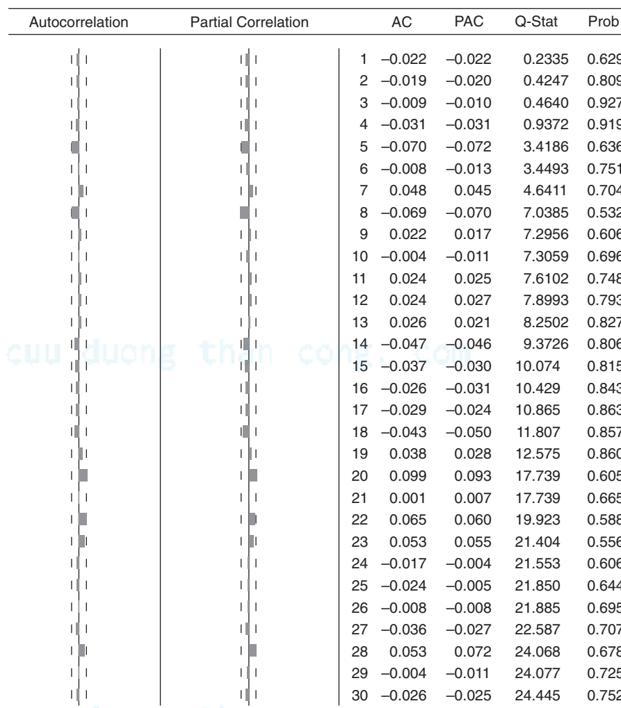
FIGURE 21.6 Correlogram of white noise error term u . AC = autocorrelation, PAC = partial autocorrelation (see Chapter 22), Q-Stat = Q statistic, Prob = probability.
