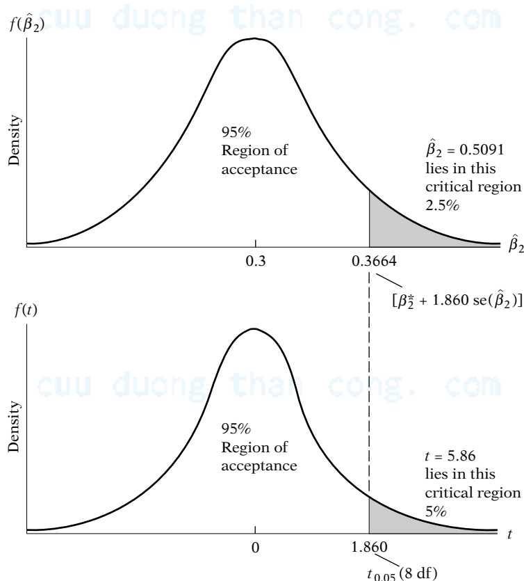
FIGURE 5.5 One-tail test of significance.
