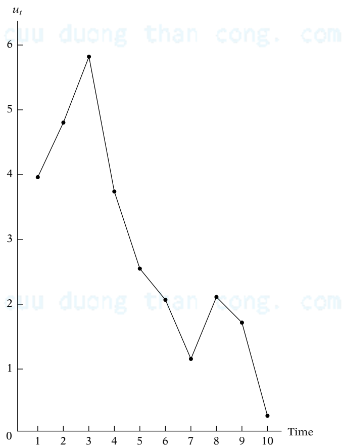
FIGURE 12.5 Correlation generated by the scheme u_t = 0.7u_{t-1} + \varepsilon_t (Table 12.1).
