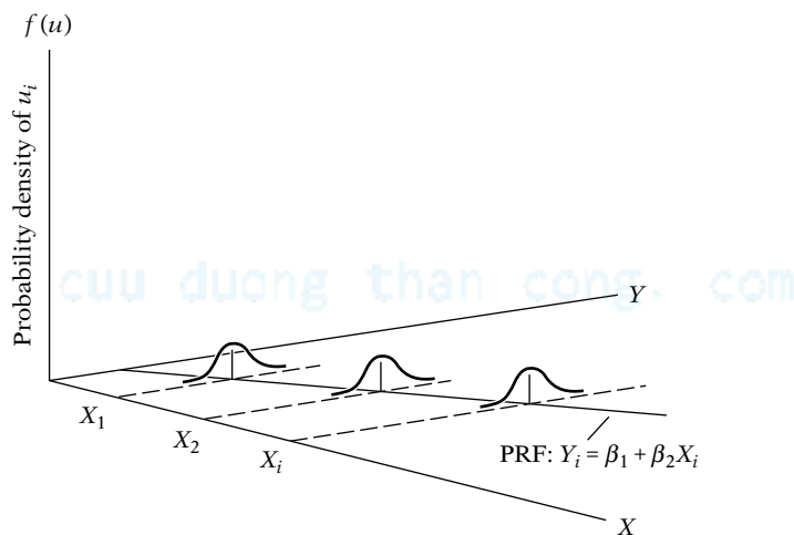
FIGURE 3.4 Homoscedasticity.
