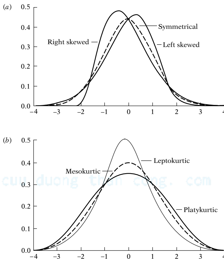
FIGURE A.3 (a) Skewness; (b) kurtosis.
