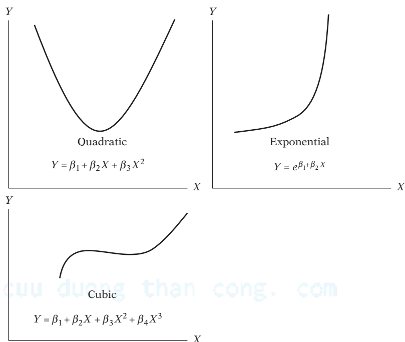
FIGURE 2.3 Linear-in-parameter functions.
