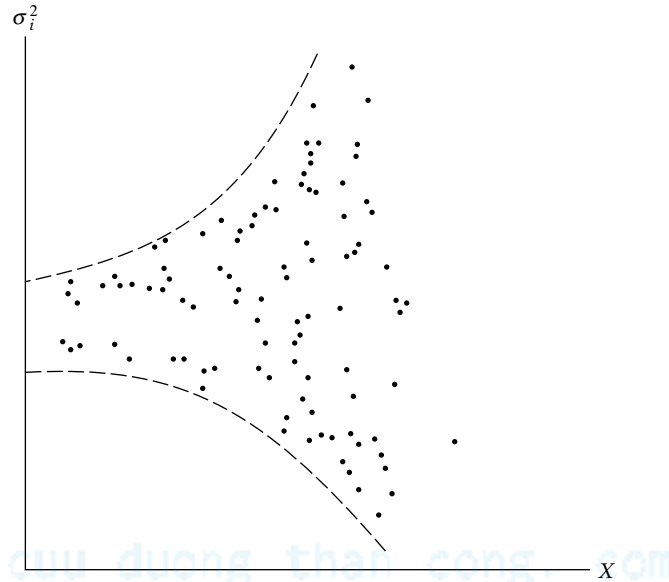
FIGURE 11.10 Error variance proportional to X^2 .
