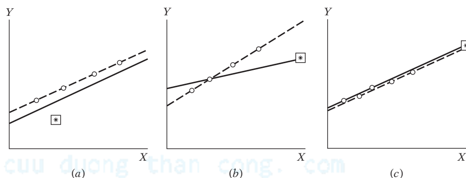
FIGURE 13.4 In each subfigure, the solid line gives the OLS line for all the data and the broken line gives the OLS line with the outlier, denoted by an *, omitted. In (a), the outlier is near the mean value of X and has low leverage and little influence on the regression coefficients. In (b), the outlier is far away from the mean value of X and has high leverage as well as substantial influence on the regression coefficients. In (c), the outlier has high leverage but low influence on the regression coefficients because it is in line with the rest of the observations.
