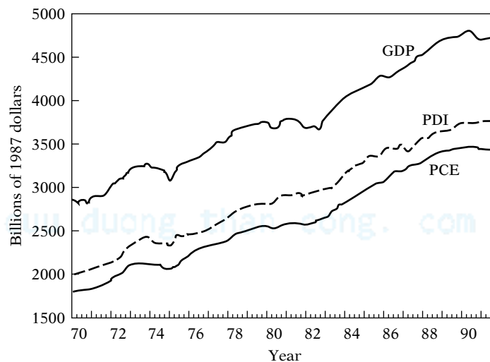
FIGURE 21.1 GDP, PDI, and PCE, United States, 1970–1991 (quarterly).
