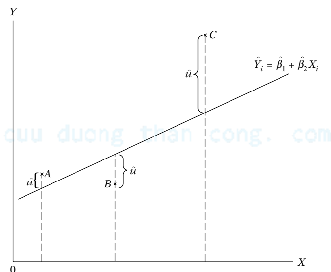
FIGURE 11.7 Hypothetical scattergram.
