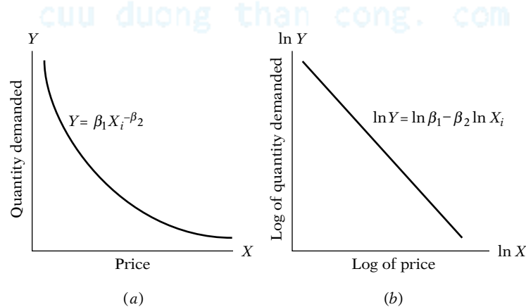
FIGURE 6.3 Constant-elasticity model.
