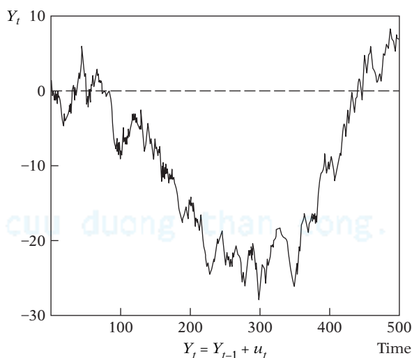
FIGURE 21.3 A random walk without drift.
