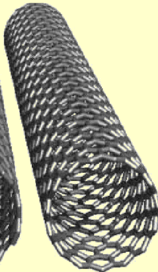
Zigzag (n,0)
