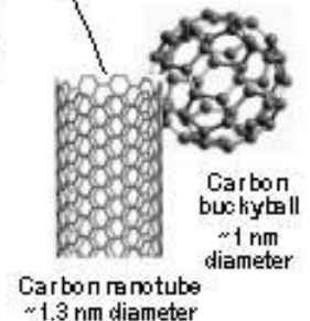
Nanotube electrode
