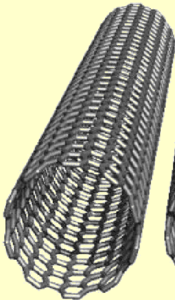
Armchair (n,n)
