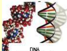
DNA ~ 2-12 nm diameter
