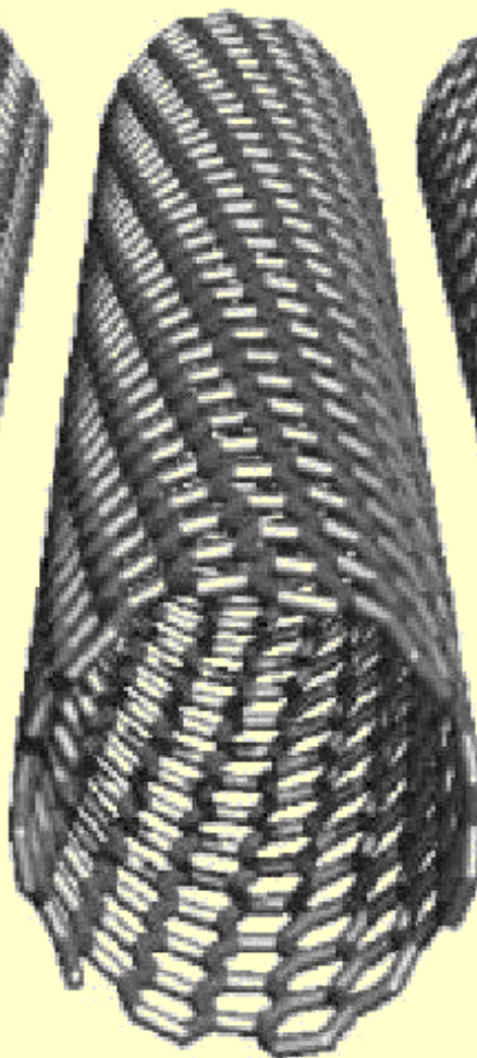
Chiral (n,m)
