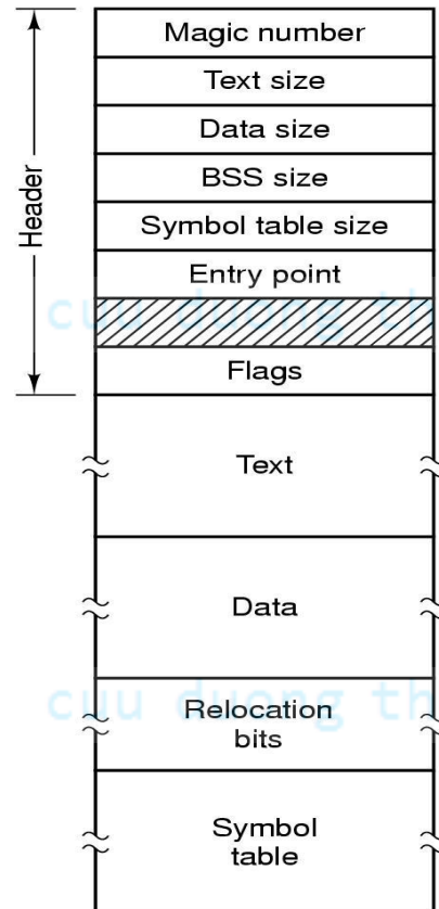
Executable file
