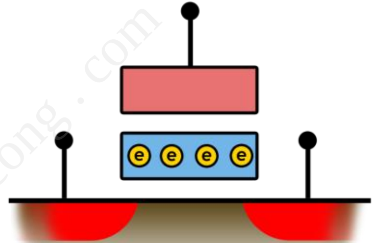
Programmed '0'
