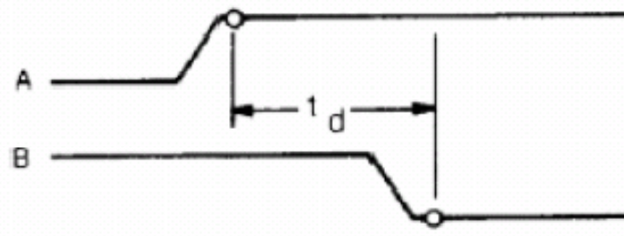
DELAY TIME BETWEEN RESULTING LOGIC LEVEL OF SIGNAL A AND RESULTING LOGIC LEVEL OF SIGNAL B
