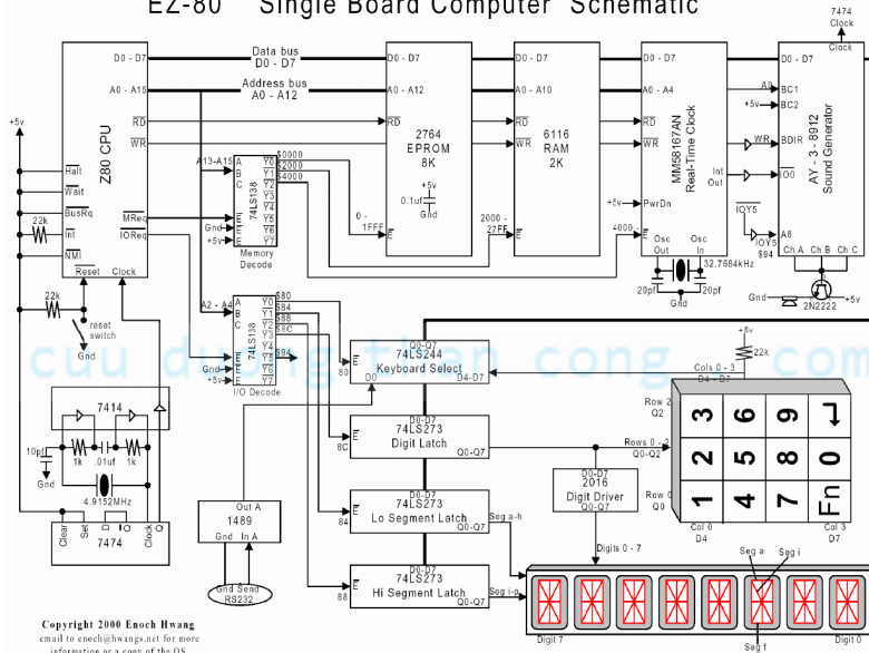
EZ-80 Single Board Computer Schematic
