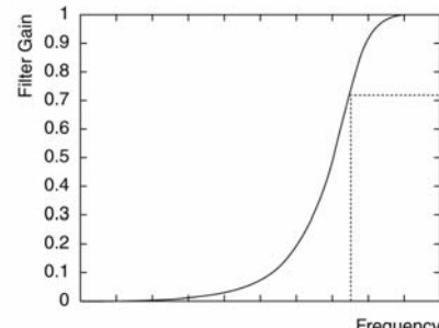
(b) High Pass Filter
