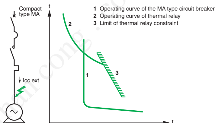
Fig. N68 : The thermal-withstand limit of the thermal relay must be to the right of the CB magnetic-trip characteristic
