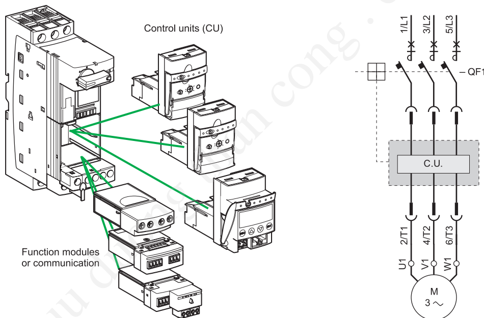
Fig. N65 : Example of a CPS modularity (Tesy U starter controller by Telemecanique)
