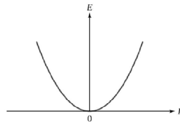
Energy momentum diagram for a free electron
