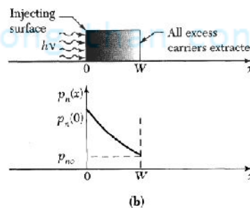
Fig. 16 Steady-state carrier injection from one side. (a) Semiinfinite sample. (b) Sample with thickness W .
